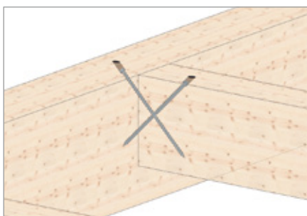
Stompe dwarsverbinding
