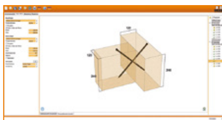
Dwarsbalk verbinding
