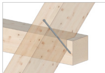
Spant-gordingverbinding
